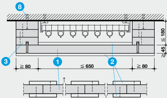
Detail G - Alternativer Deckenkanal
